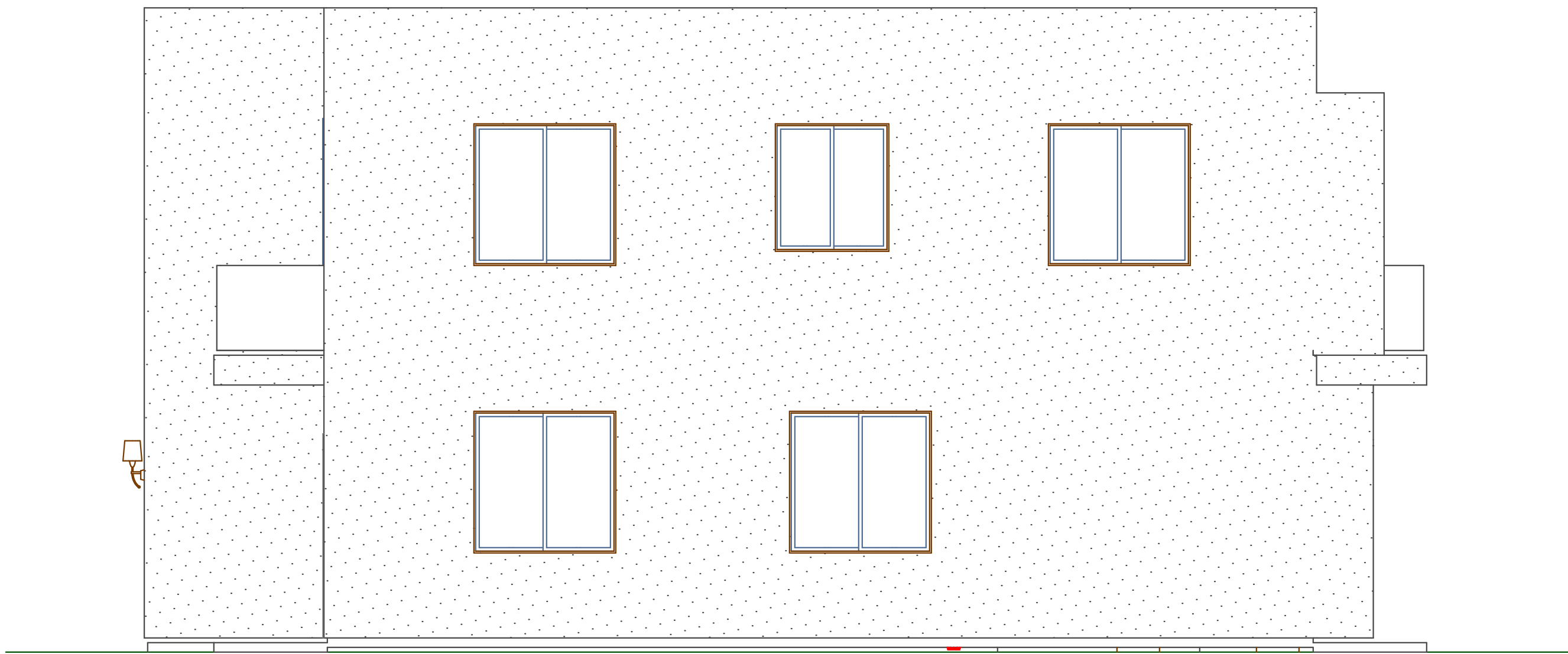
E8 Right Elevation SCALE: 1/4" = 1'-0"
