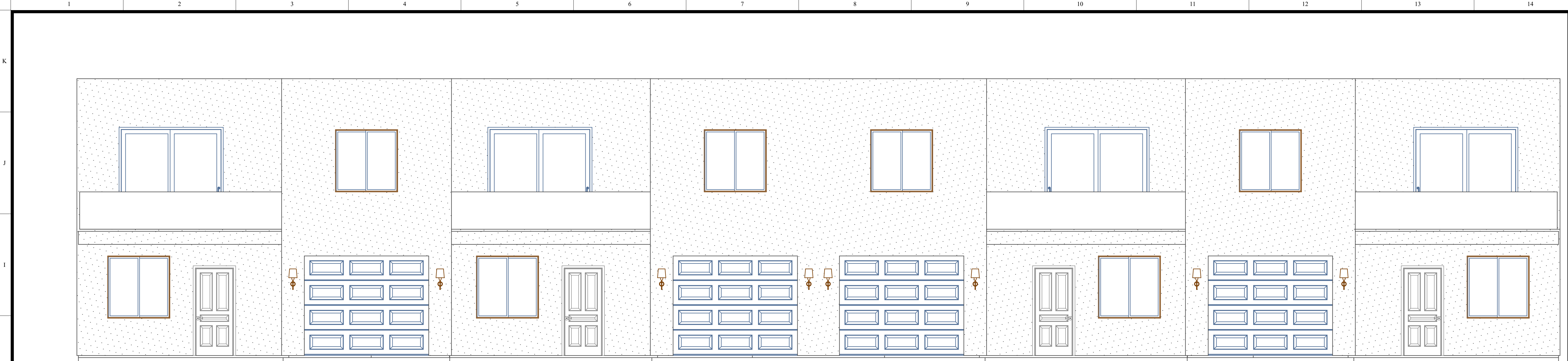
H1 Front Elevation SCALE: 1/4" = 1'-0"
