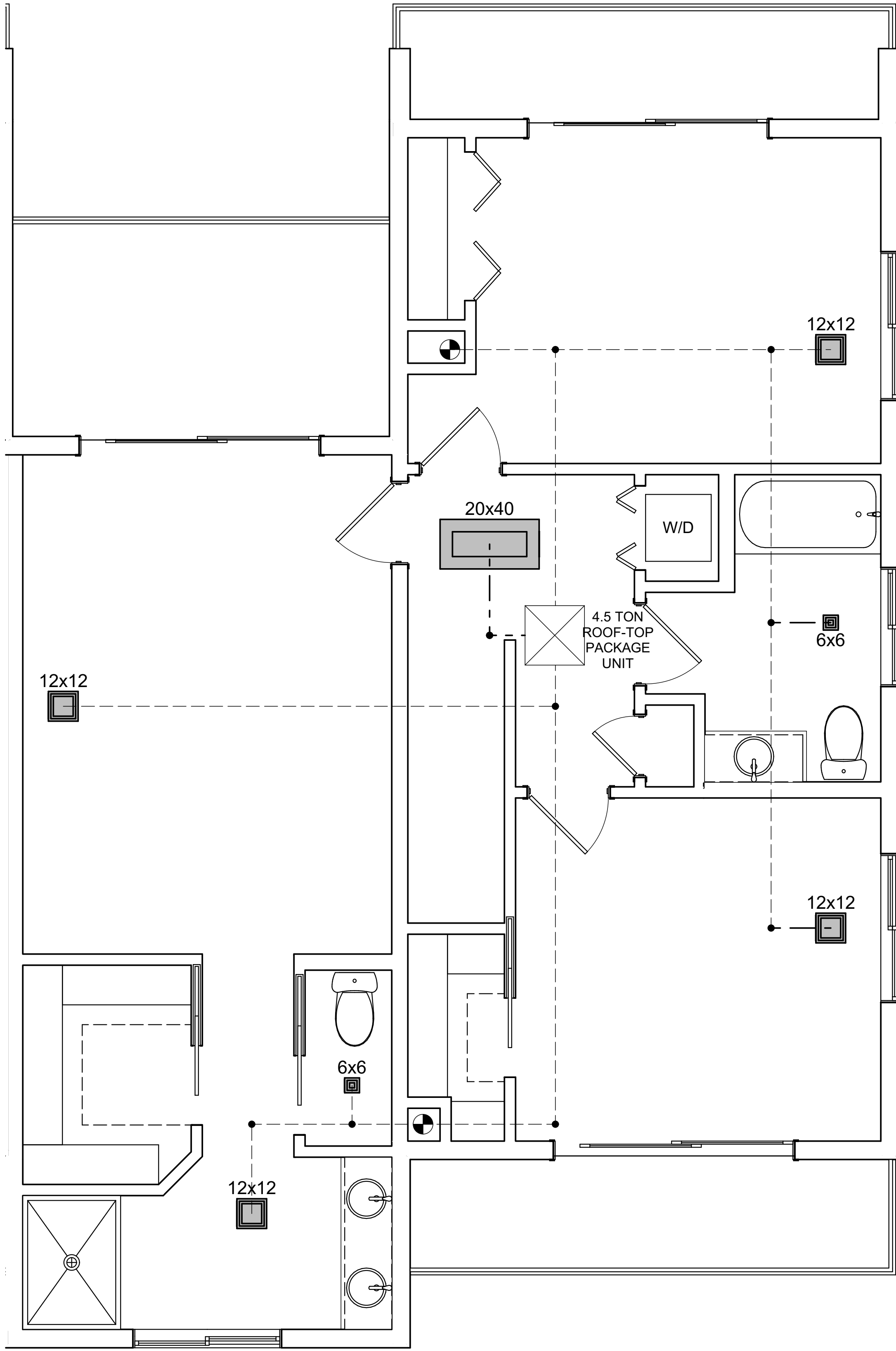
B7 Typical Second Floor HVAC
