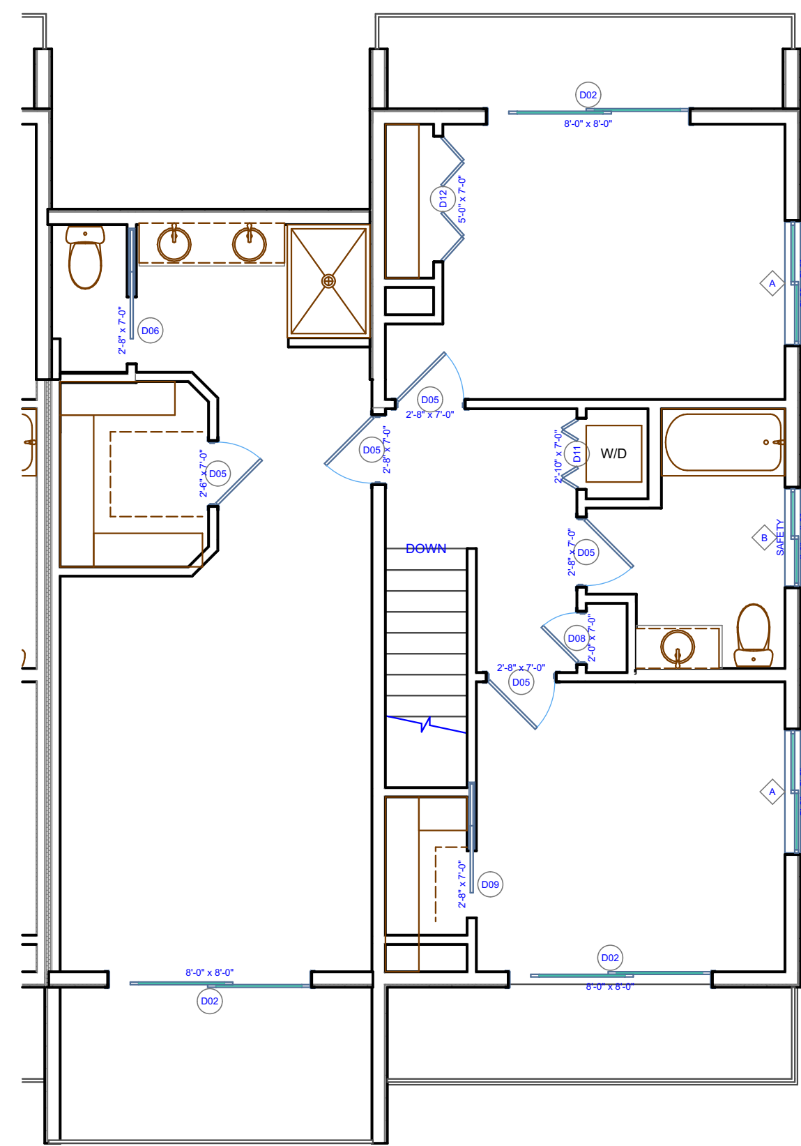
A12 Alternate Master Bedroom SCALE: 3/16" = 1'-0"
