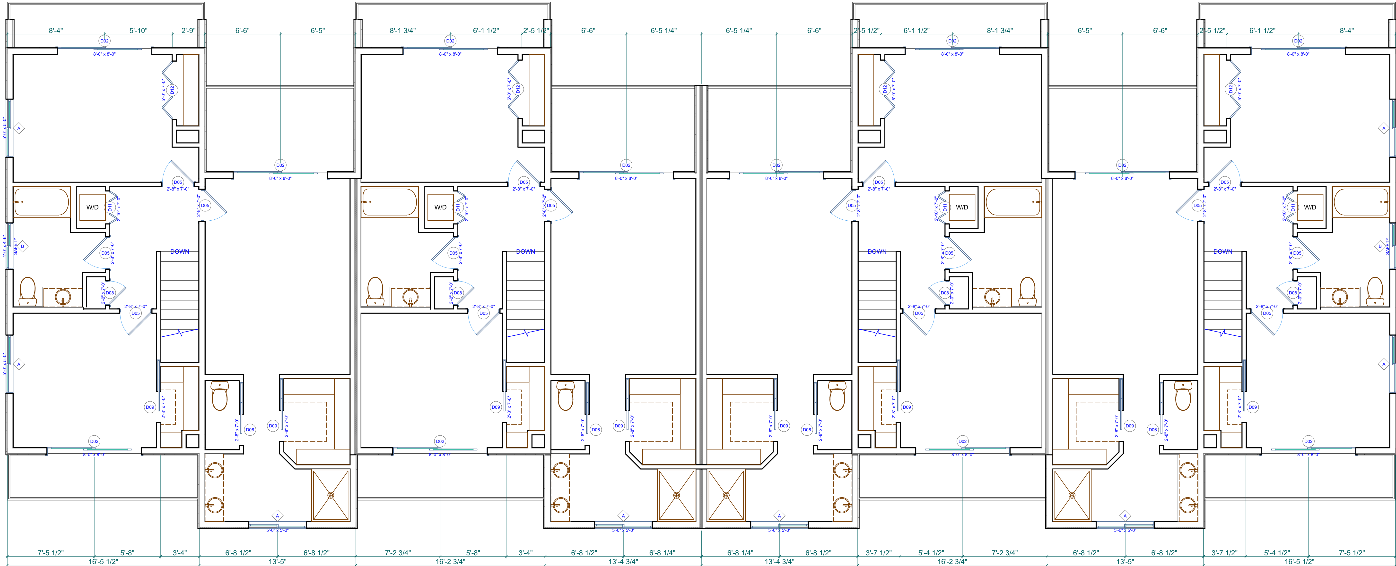
E1 Second Floor Plan SCALE: 1/4" = 1'-0"
